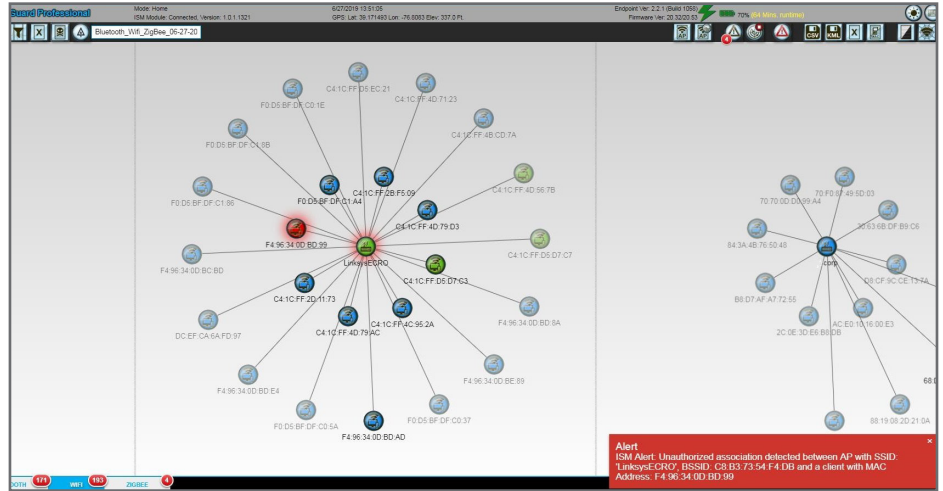
Spider Chart
